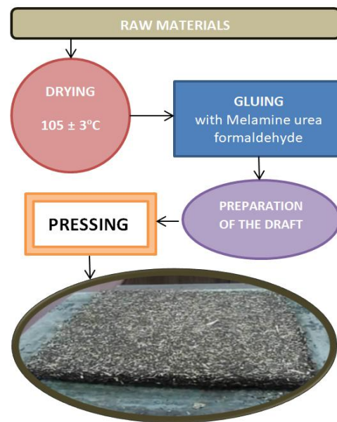
Figure 9. Hot pressed plate draft (adapted from [36])
