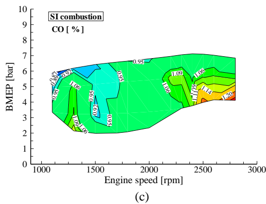
Figure 6. Emissions and exhaust gas temperature (a) exhaust gas temperature, (b) NO x , (c) CO, (d) HC emissions
