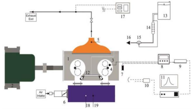
(1)Test engine, (2)dynamometer, (3) in-cylinder pressure sensor,(4)spark plug, (5)exhaust gas temperature-thermocouple, (6) throttle (7) encoder, (8) amplifier (9) oscilloscope, (10) data logger, (11) computer, (12) port injector system, (13) fuel tank, (14) scaled container, (15) regülötör, (16) fuel pump, (17) gas emissions device, (18) termocouple for intake air temperature, (19) pressure sensor.
