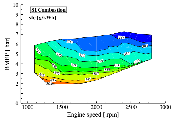
Figure 4. Specific fuel consumption(sfc) map of the engine.
